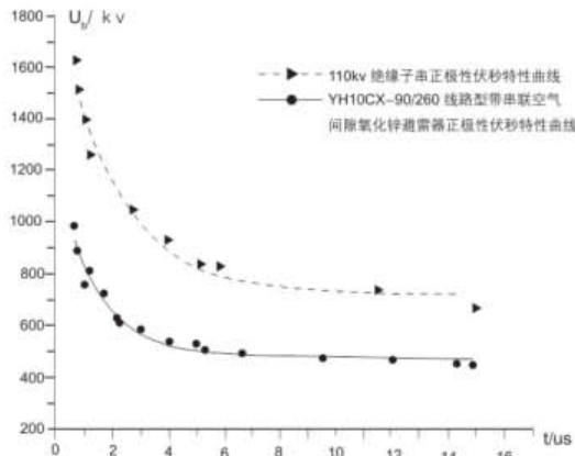
图 22 110kV 绝缘子串与纯空气间隙线路避雷器的伏秒特性配合曲线 Fig22 V-S characteristic coordination curve of the insulator string with single air gap the arrester for 110kV
