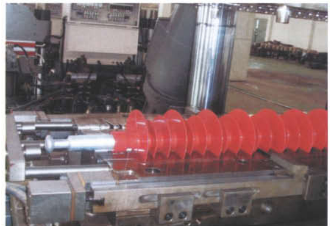
注射硫化 Injection & sulfuration
