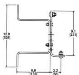
Pole Mounting bracket 柱上安装支架
